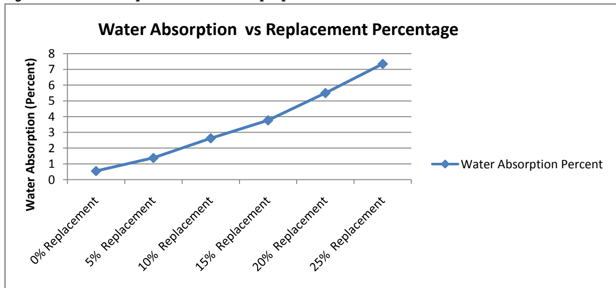
Figure 3 Water Absorption at various mix proportions
